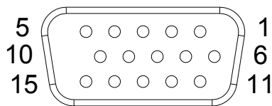
Figure 2.24 VGA Connector
